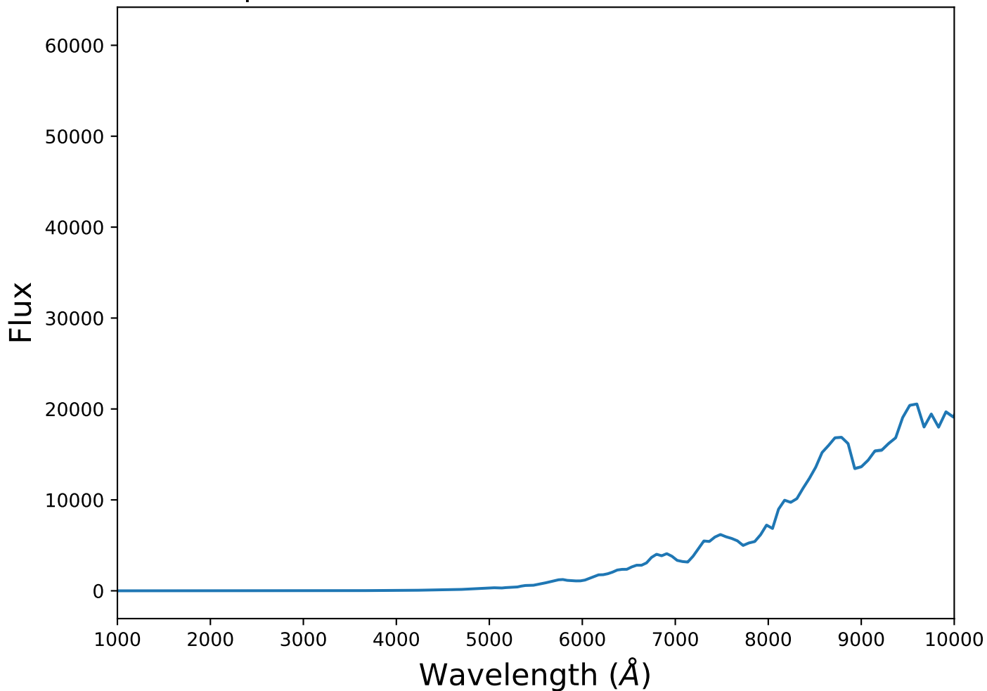
Spectrum 2 for transient PISNb at z=0.49
